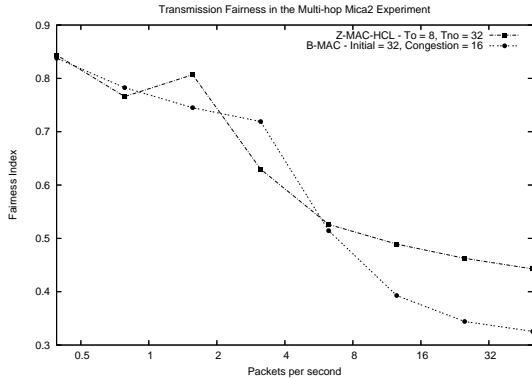
Figure 13: Fairness index from the multi-hop Mica2 benchmark
