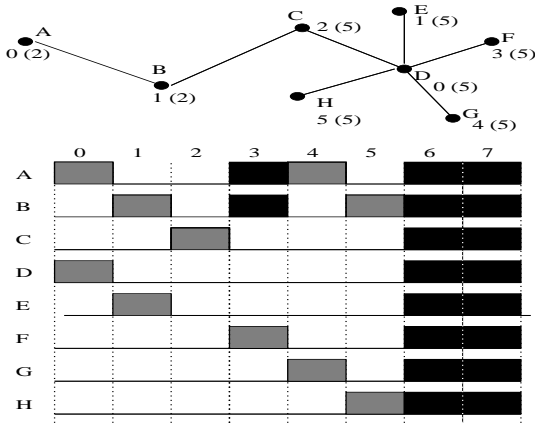
Figure 1: An example of the TF rule. The top figure shows a network topology and the numbers indicate the slot numbers assigned by DRAND and the numbers in parenthesis are F_i . The bottom figure shows the slot schedule of all nodes (shaded slots are ones where each node transmits, and dark slots are the “empty” slots that are not used by any one-hop or two-hop neighbors).
