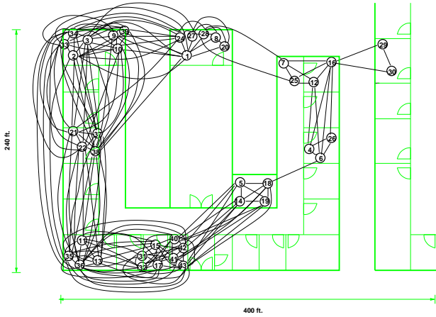
Figure 3: NCSU testbed with 42 Mica2 nodes.
