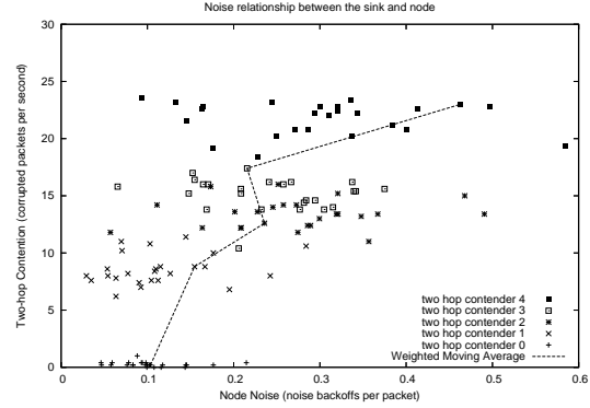
Figure 2: The correlation between noise level and two-hop contention.
