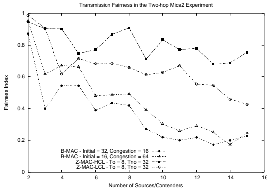
Figure 12: Fairness index from the two-hop Mica2 benchmark
