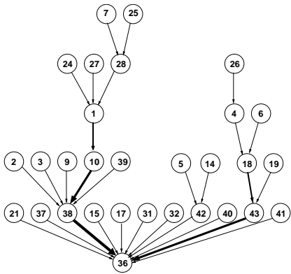
Figure 4: Routing paths used in the multi-hop Mica2 benchmark.
