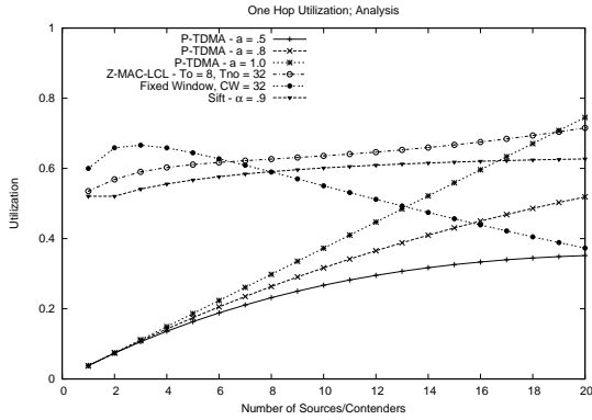
Figure 7: The analytical data throughput comparison in the one-hop benchmark
