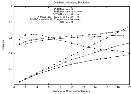
Figure 6: The data throughput comparison in the one-hop ns-2 benchmark.
