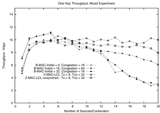
Figure 5: The data throughput comparison in the one-hop Mica2 benchmark.
