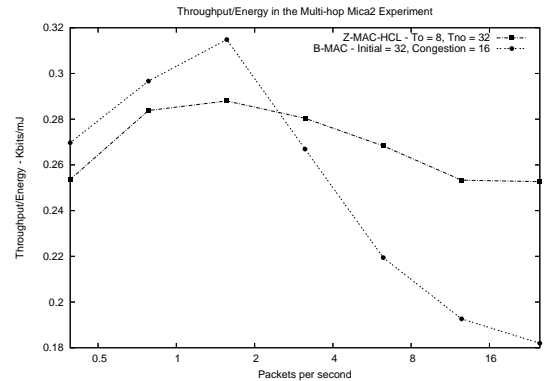
Figure 15: The power efficiency in the multi-hop Mica2 benchmark.
